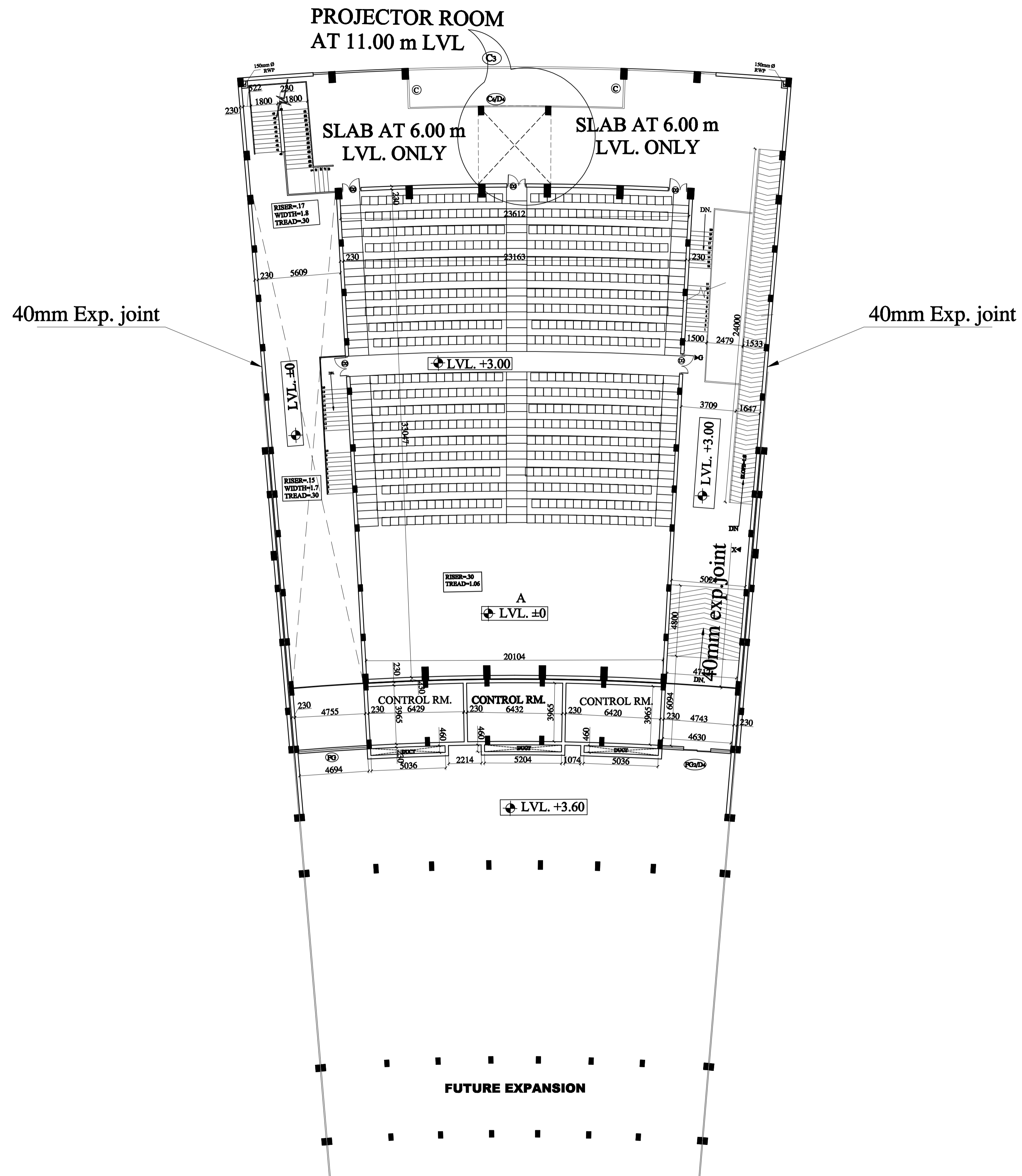
PLAN OF 600 SEATER LECTURE HALL (LHTC)
